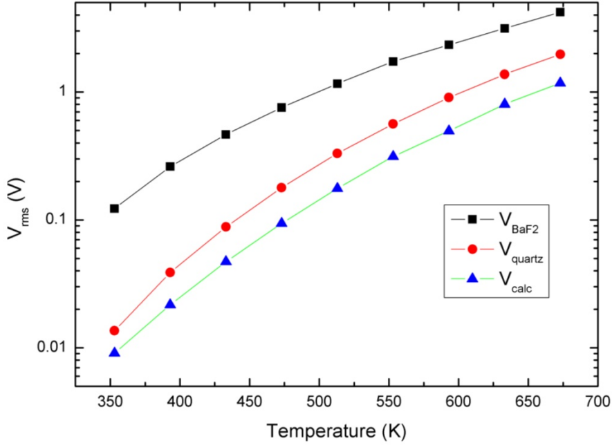
Figure 5: Effect of window material on the signal produced by the pyroelectric detector. Data collected using the \text{BaF}_2 window (black squares) and fused-quartz window (red circles) are plotted as a function of the temperature of the hollow graphite rod that was used as the target. The blue triangles are calculated values for fused-quartz window using Eq. 3.
